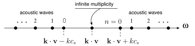
Figure 1: Spectrum of disturbances without shear flow
