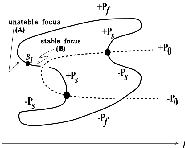
Figure 6: The bifurcation diagram on the equilibria of (4.3) when the parameter moves along the arrow l in Fig5.
